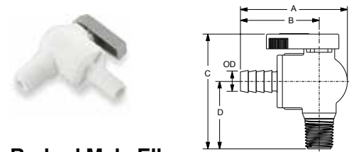
VME - Valve Barbed Male Elbow
